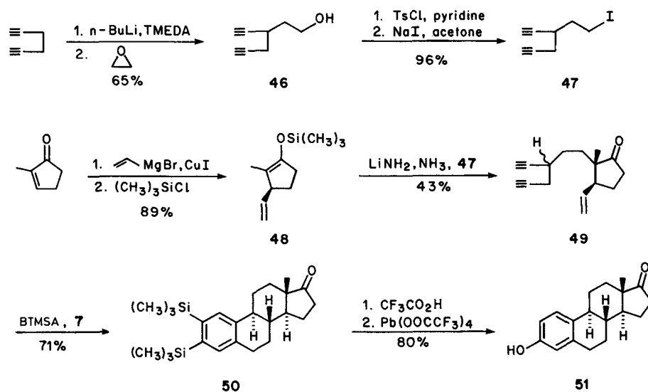
Scheme 23. A \text{CpCo}(\text{CO})_2 -catalyzed synthesis of (±)-estrone.
