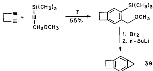
Scheme 17. \text{CpCo}(\text{CO})_2 -catalyzed synthesis of 3,4-dihydro-1 H -cyclobuta[a]cyclopropa[d]benzene 39 .
