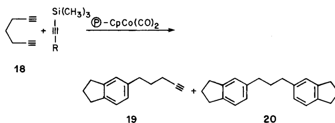
Scheme 11. Catalytic cyclization of 1,6-heptadiyne by polystyrene-supported \text{CpCo}(\text{CO})_2 . \text{P} = \text{polystyrene} .
