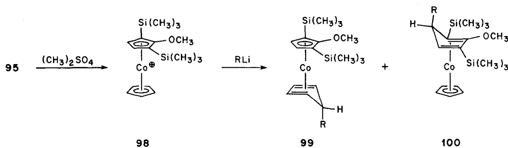
Scheme 46. Nucleophilic additions to cobaltocenium salts.
