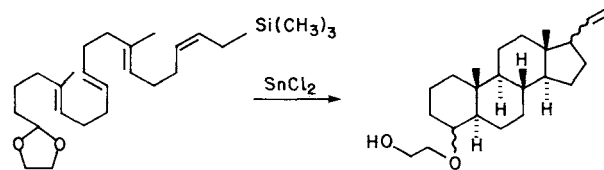
Scheme 1. Polyene cyclization according to Johnson et al. [2].
