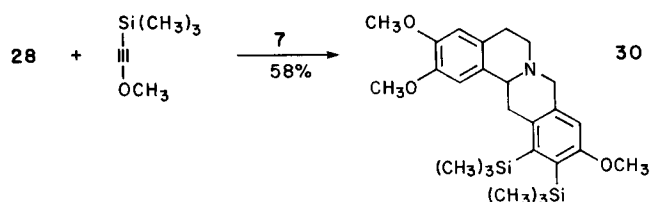
Scheme 14. Regioselective protoberberine synthesis.
