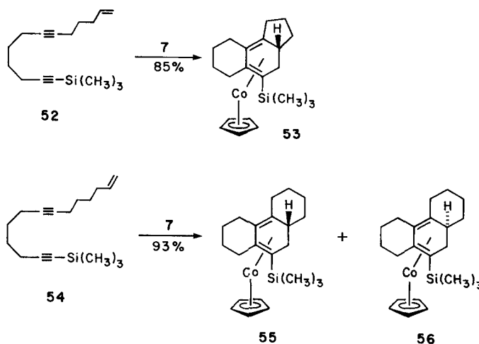
Scheme 24. Intramolecular cyclizations of enediynes with terminal double bonds.
