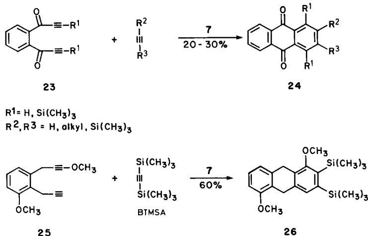
Scheme 12. Two cyclization strategies for the preparation of anthraquinones.
