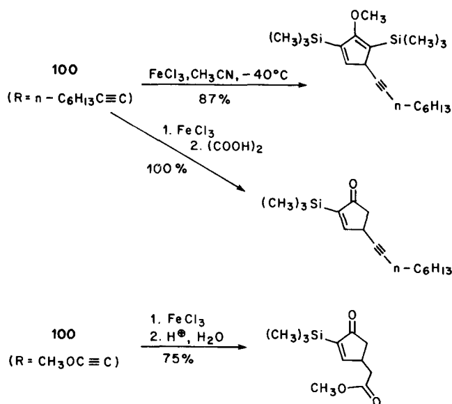
Scheme 47. Oxidative decomplexation of the substituted ligands in 100 .
